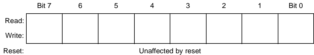
Figure 8-2. Accumulator (A)
