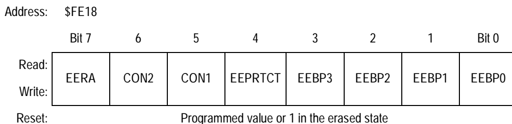
Figure 7-2. EEPROM-2 Non-Volatile Register (EENVR2)
